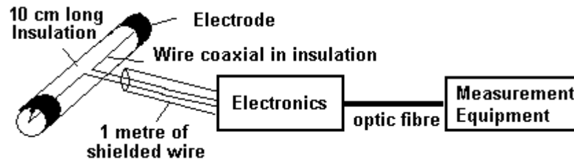
Figure 4.1: Low input impedance electric field sensor system
