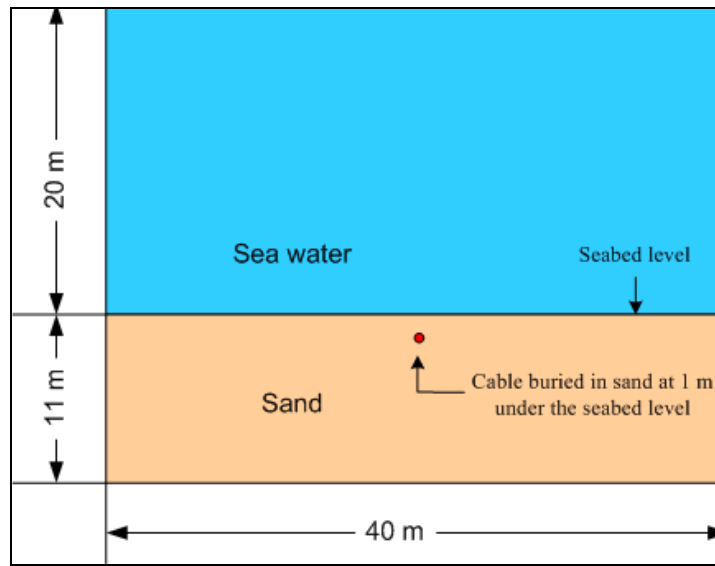
Figure 3.3: Cabling scenario of the submarine cable used in simulations (where m = metres)
